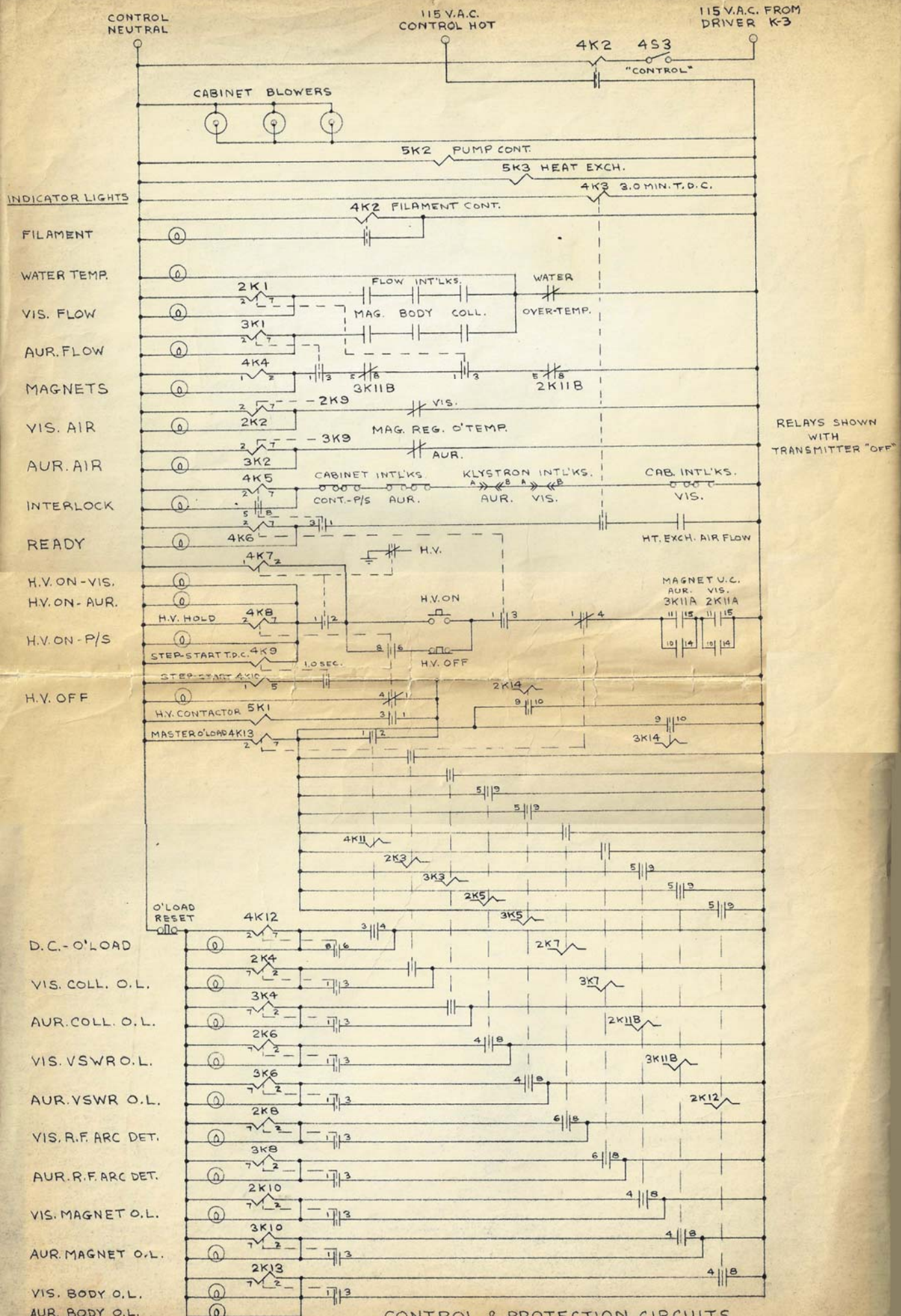
CONTROL & PROTECTION CIRCUITS KLYSTRON POWER AMPLIFIERS KHOF-TY TRANSMITTER
